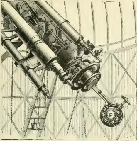
FIG. 14.—Spectroscope attached to a large refractor which throws an image of the sun on the slit plate.
